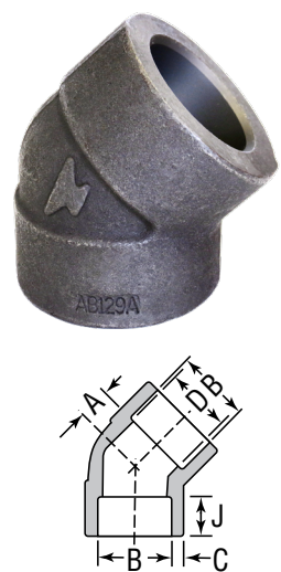
Figure 2171 45° Elbows
