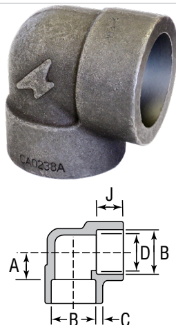
Figure 2170 90° Elbows
